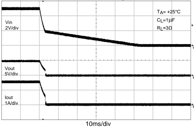
UVLO Decreasing
